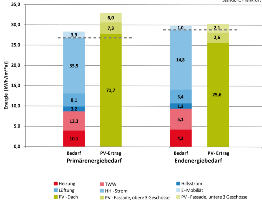
Figure 3: Final- and Primary Energy Balance, Location Frankfurt, Date: 22.10.12; Source: Steinbeis-Transferzentrum, EGS-plan, Stuttgart
