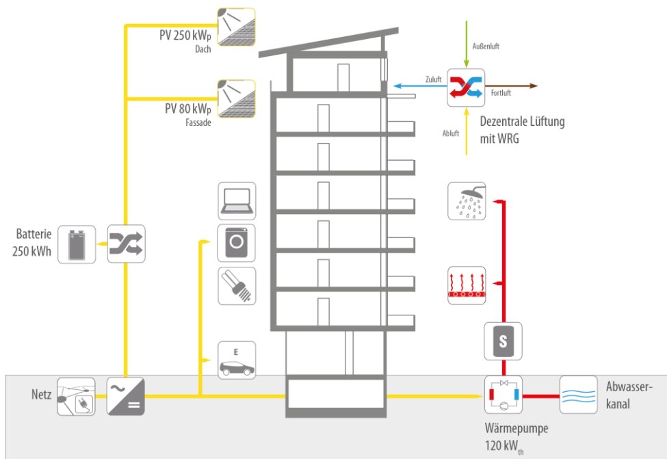
Figure 2: Energy Flow Schematic, Aktiv-Stadthaus; Source: Steinbeis-Transferzentrum, EGS-plan, Stuttgart
